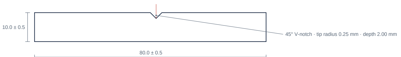
Fig. 3 ISO 179-1 Charpy notched specimen 80 \times 10 \times 4 mm, 45° V-notch, depth 2.0 mm
